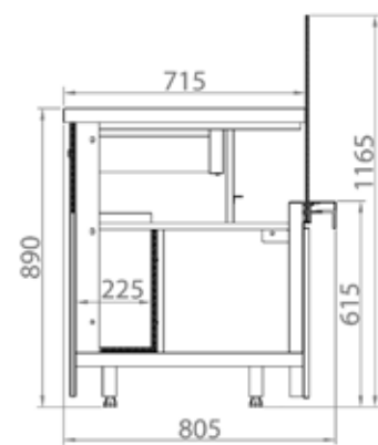
094 CUBE till module with money case L= 625, 1250 mm
